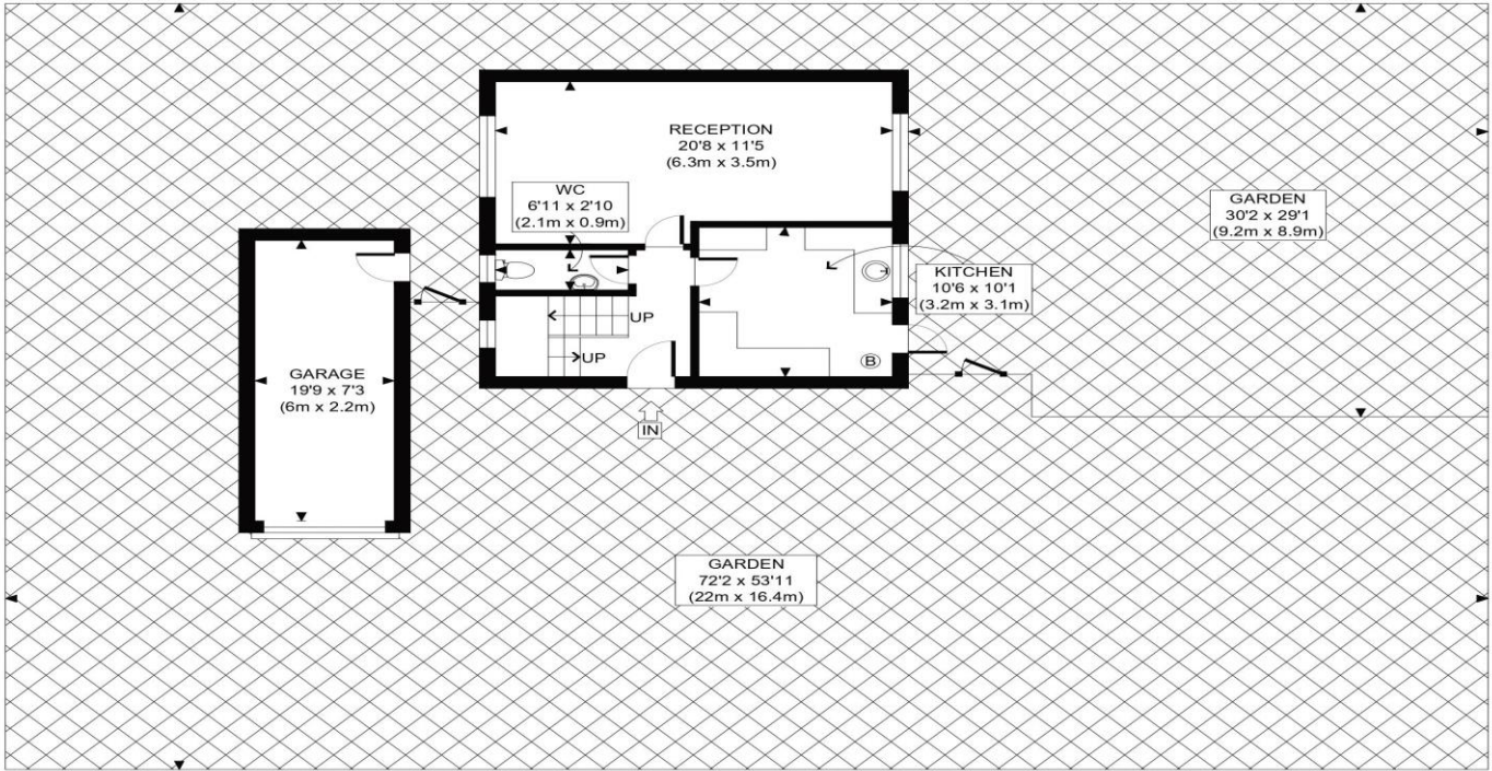
GROUND FLOOR GROSS INTERNAL FLOOR AREA 429 SQ FT
